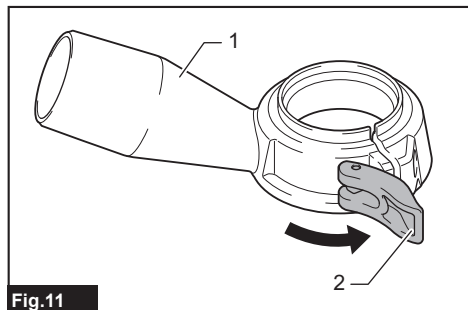
Fig.11 ► 1. Dust extraction attachment 2. Clamp lever
