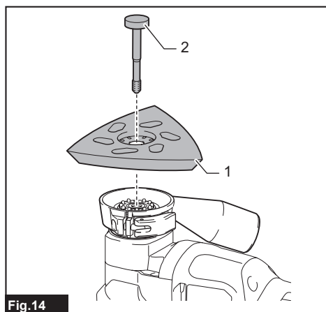
Fig.14 ► 1. Sanding pad 2. Holder bolt
